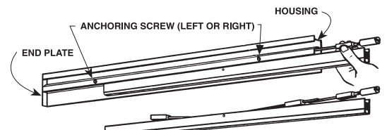
Figure 1 - Reversing the Mechanism
