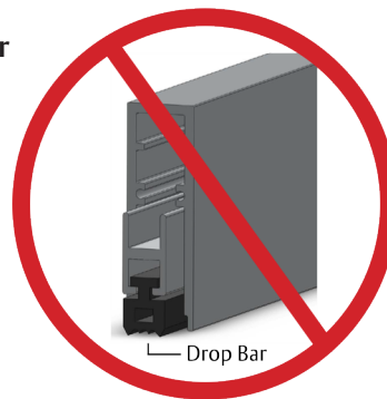
Figure 3 - Improper Drop Bar This shows an improper drop bar protruding from the end of the case. The drop bar should be flush at both ends.
