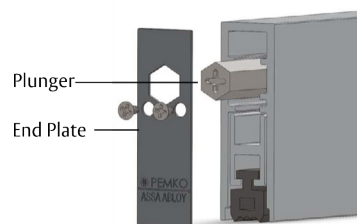
Figure 5 Plunger end plate prevents the plunger adjustment from rotating.
